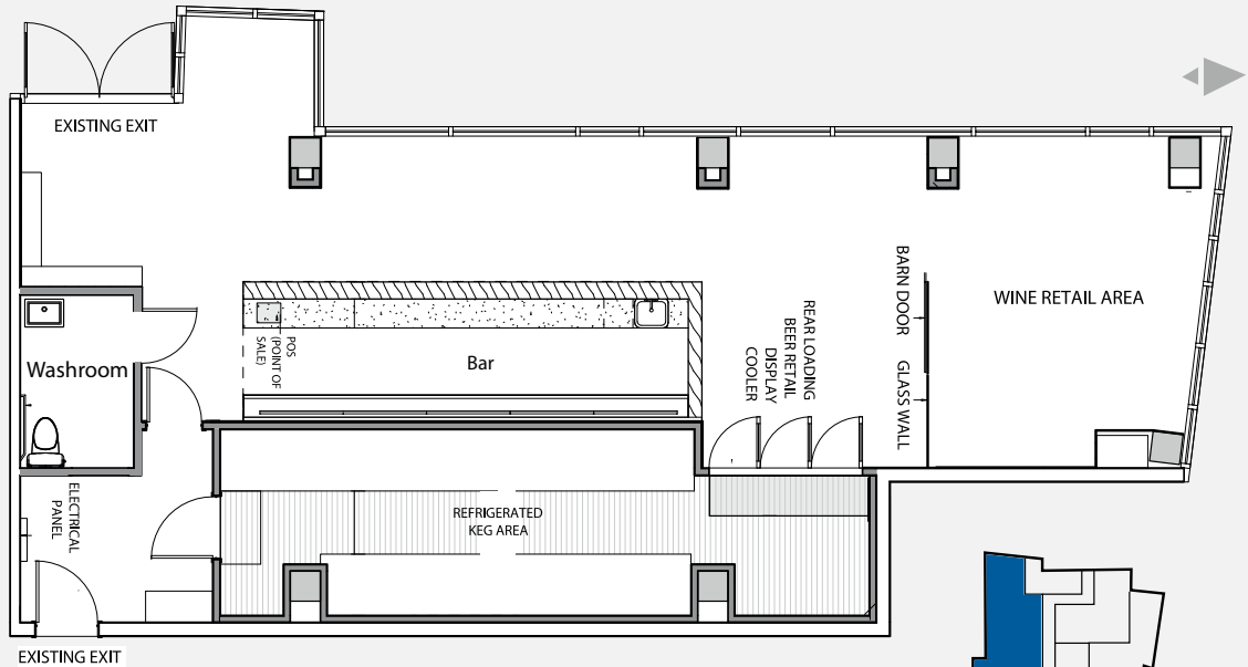
EXISTING LAYOUT
